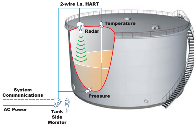
Example Tank Gauging System
