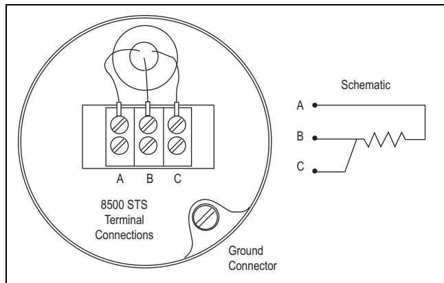
8500 STS connection
